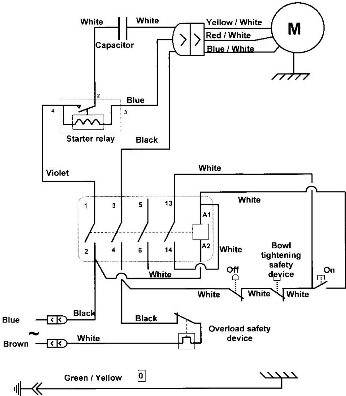
Electrical wiring diagram 220-240V 50/60Hz
